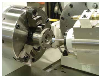
Ball nut on GS:TI-LM Universal Grinder
